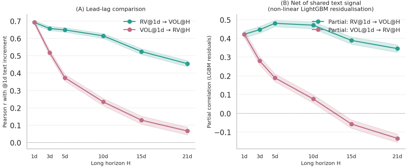
Figure 8: Lead-lag asymmetry between text-driven uncertainty and trading activity
