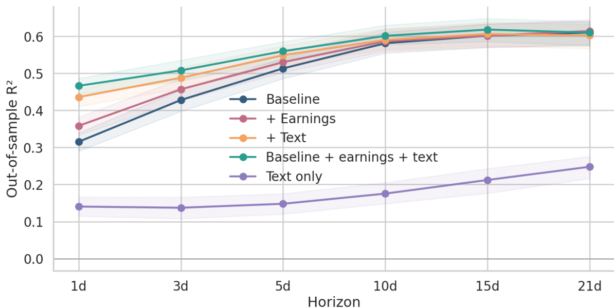
Figure 4: Realised variance
